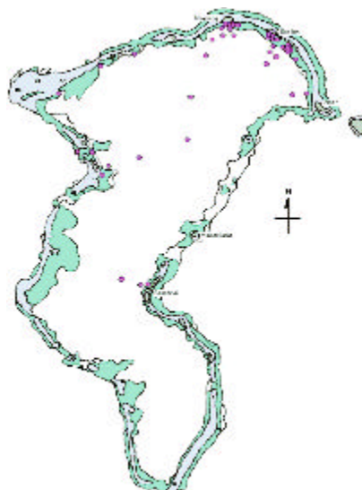
Fig. 2. Sea truth points at Ulithi atoll
