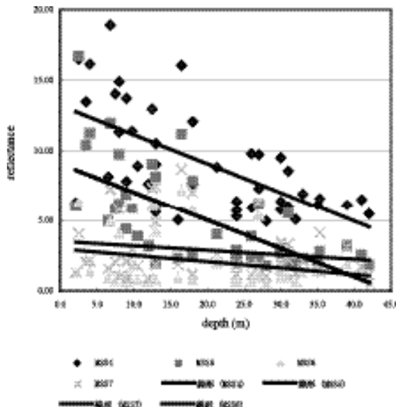
Fig. 5. Relationships between sea depth and mean reflectance corresponded with Landsat/MSS band
