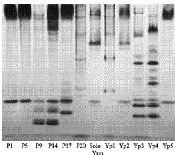
Fig. 1. Different band pattern of tuber protein of yam collected from Pohnpei island and Yap Proper by NON-SDS polyacrylamide gel electrophoresis
